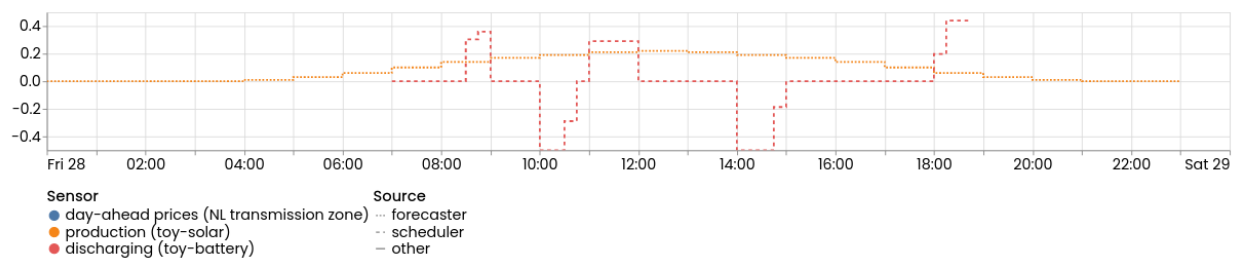
Power (MW)
